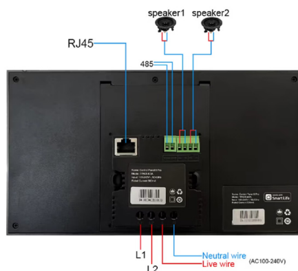
Product wiring diagram
